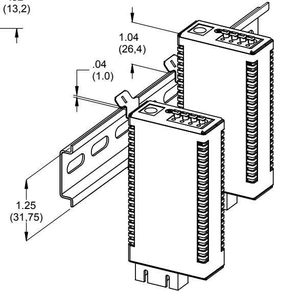
DIN Rail Mounting Positions
